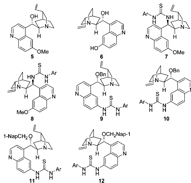
Figure 1. Catalysts screened for the Mannich reaction (Ar = 3,5-(CF 3 ) 2 C 6 H 3 –; 1-Nap = 1-naphthyl).
