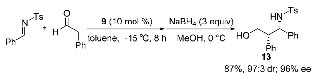
Scheme 1. Mannich Reaction between N -Tosylimine and Phenylacetaldehyde
