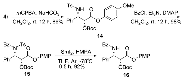
Scheme 2. Synthesis of Protected Paclitaxel Side Chain
